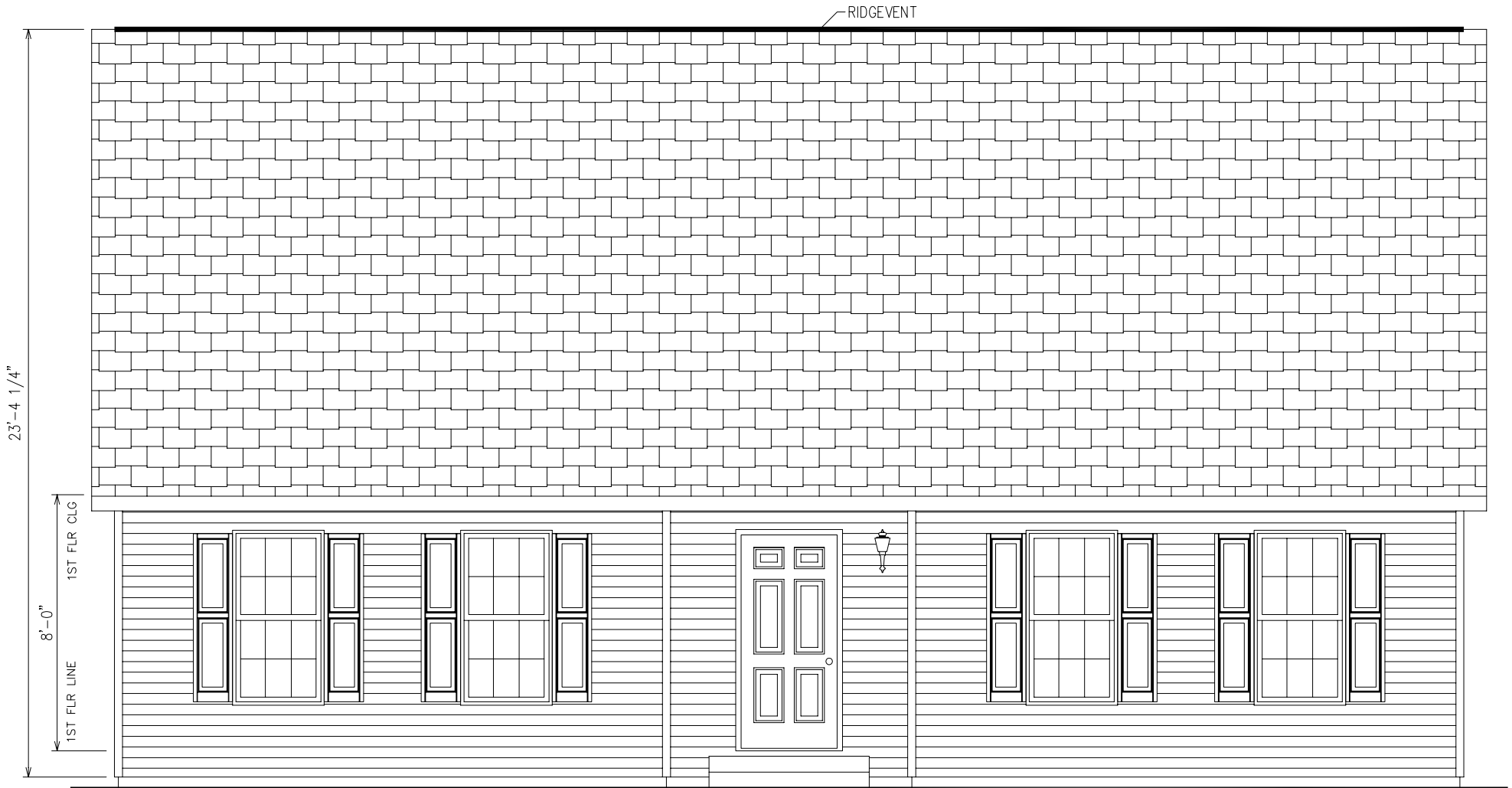
FRONT ELEVATION
