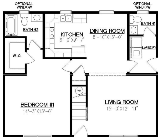
First Floor (w/ Crawl Space)
